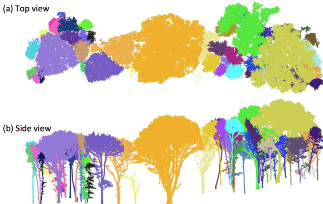
Figure 2.4 Example of a co-registered and segmented TLS point cloud from Wytham Woods, UK. Single trees extracted for a 20 x 100 m transect. Data captured with a RIEGL VZ-400 instrument and tree extraction was done with the treeseq algorithm (Burt et al., 2019). (a) Top view; (b) Side view
