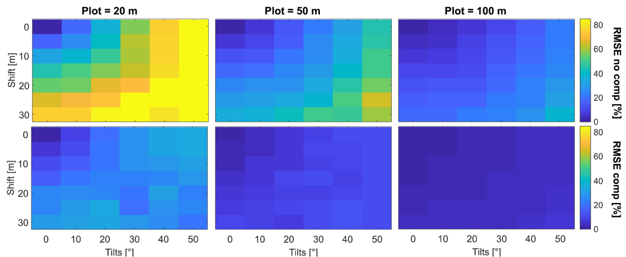
Figure 3.3 Joint effect of plot size (Plot), sensor angle incidence (Tilt) and geolocation error (Shift) on difference in total crown volume estimated by an active remote sensor and the same volume as generally measured from the ground with trunk-based measurements. The sensor's footprint is identical to the plot size. The top row only considers the volumes of the trees measured within the plot and the bottom row also considers the volumes of the trees surrounding the plot, allowing for error compensation.
