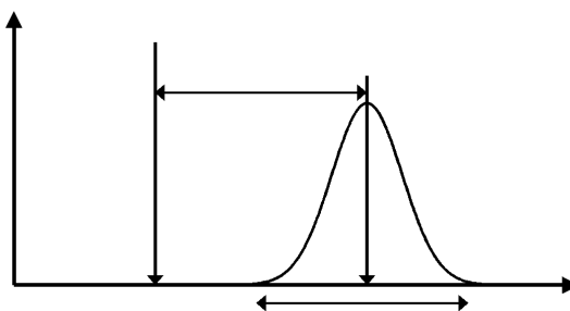
Figure 4.1 The accuracy of an estimate comprises two components. (i) Precision quantifies the variability around the estimated value. (ii) Bias quantifies the degree to which the estimated value deviates from the true (but often unknown) population value.
