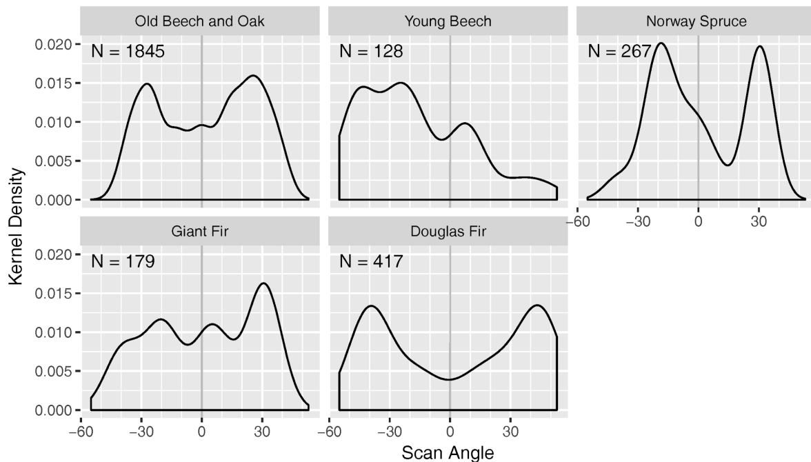
Figure 2.2 Scan angles distribution for points on the stem at DBH. Especially scan angles of >30 degrees contribute (Brede et al., 2017)
