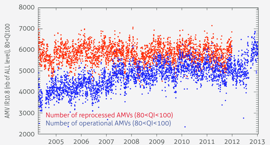
Number of wind vector products extracted from Meteosat imagery with a quality index above 80%, for reprocessed (red) and real time products (blue) in the period 2005-2013
