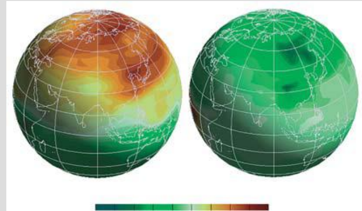
Simulated CO 2 distribution as observed by GOSAT by National Institute for Environmental Studies
