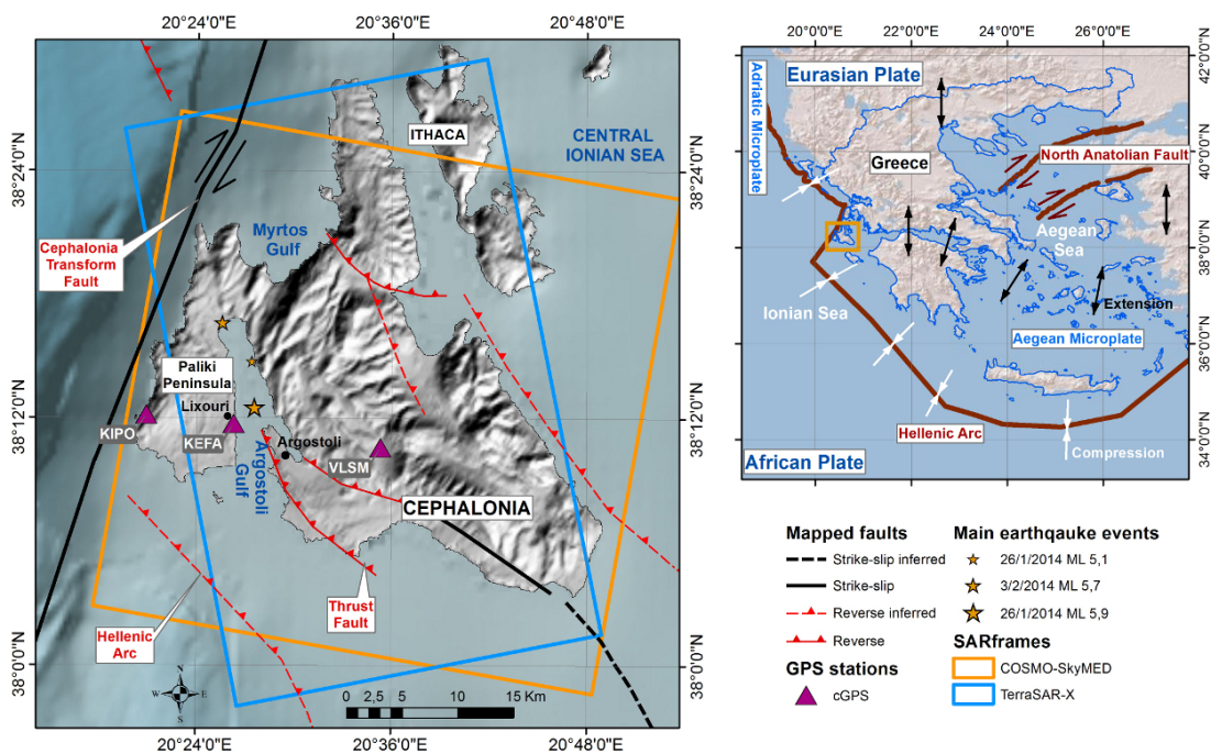
Fig. 1 Tectonic context of the Aegean Sea and the main known active faults on the island of Cephalonia. Rectangles indicate the coverage of the satellite radar images. Magenta triangles represent permanent GPS stations. Yellow stars indicate the epicenters of the three largest events of the 2014 sequence.
