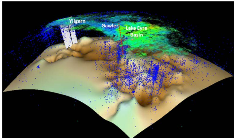
Figure 1: 3D oblique view of the Australian crust that combines the surface clay mineral composition from ASTER (warmer colours are illite-montmorillonite and cooler colours are kaolinite) with the base of crust (MOHO) and seismic activity (blue dots). http://www.ga.gov.au/data-pubs/interactive-3d-models/world-wind-3d-data-viewer
