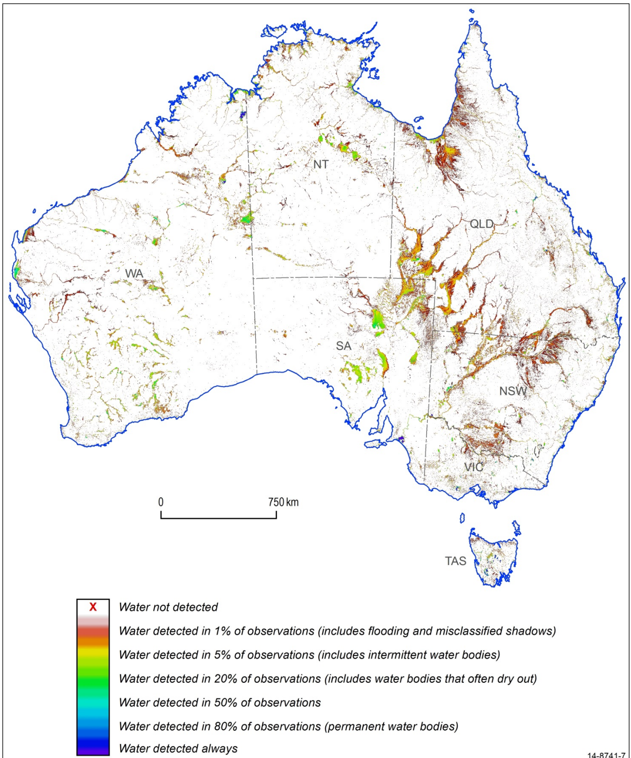
Figure 1: The Water Observations from Space (WOfS) product for all of Australia. The colouring indicates the frequency with which surface water has been observed by the Landsat 5 and Landsat 7 satellites since 1987. Most of the large water areas shown are in red to green colouring, demonstrating that while large areas may become inundated, the frequency of inundation is very low, with most of the continent usually being very dry. Most permanent water bodies, coloured blue, are too small to be visible in the Figure.
