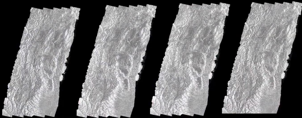
SIGMA0_HH
