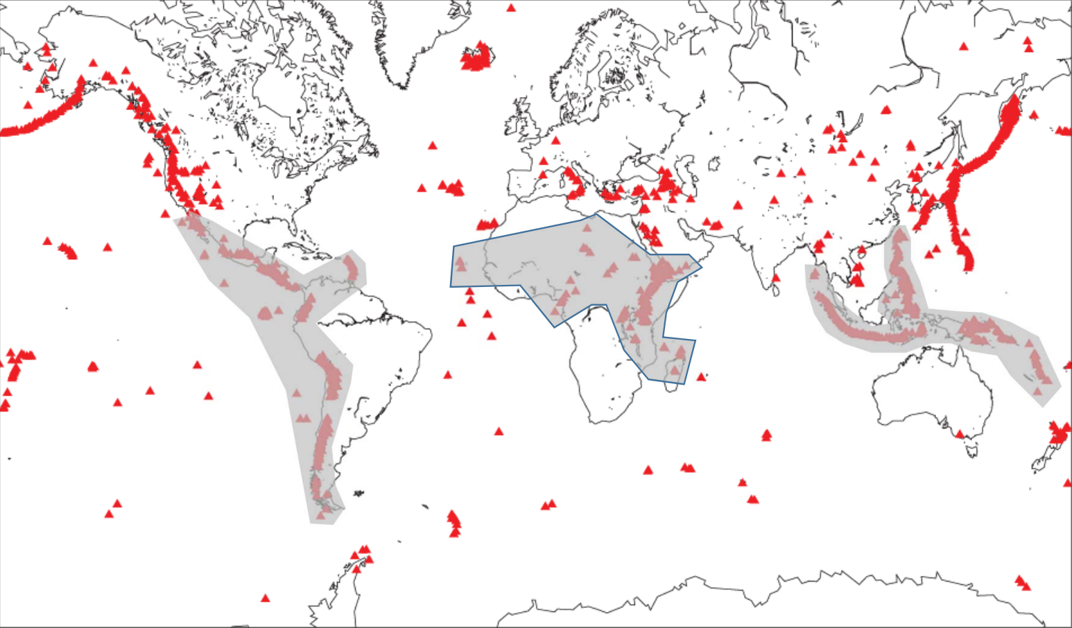
Map of volcanoes with Holocene eruptions
