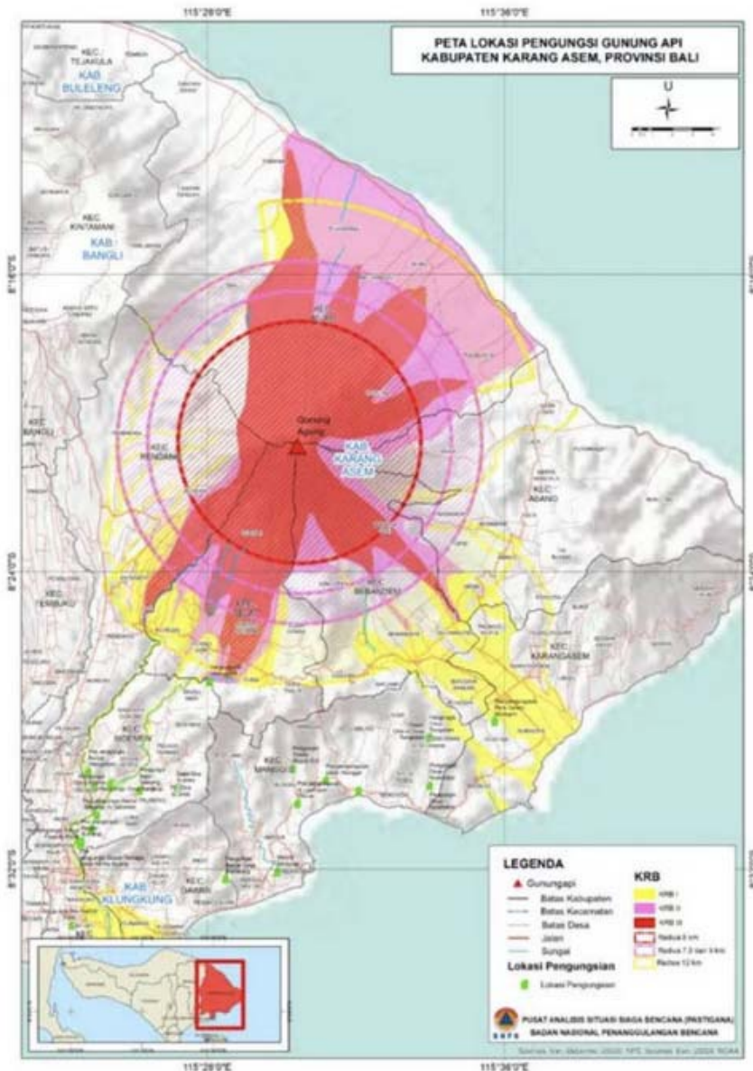
Volcanic hazards map, Agung volcano, Bali, Indonesia
